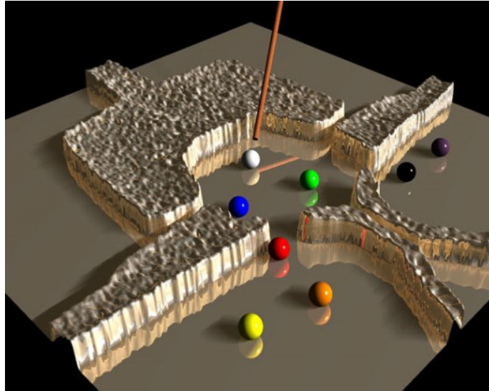
An illustration of a "quantum billiard"
